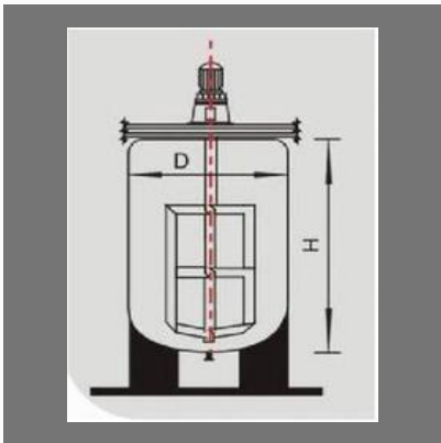
FRP Storage Tanks (Vertical, Double Seal Heads)
